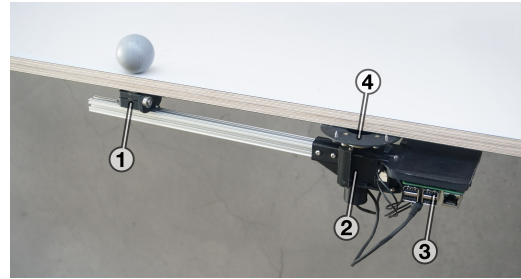
Figure 5: The robotic arm is constructed of a 25 cm metal rod with a magnet at the edge (1), an MX-28 Dynamixel motor (2), a Raspberry Pi controller (3), all mounted under the table (4).
