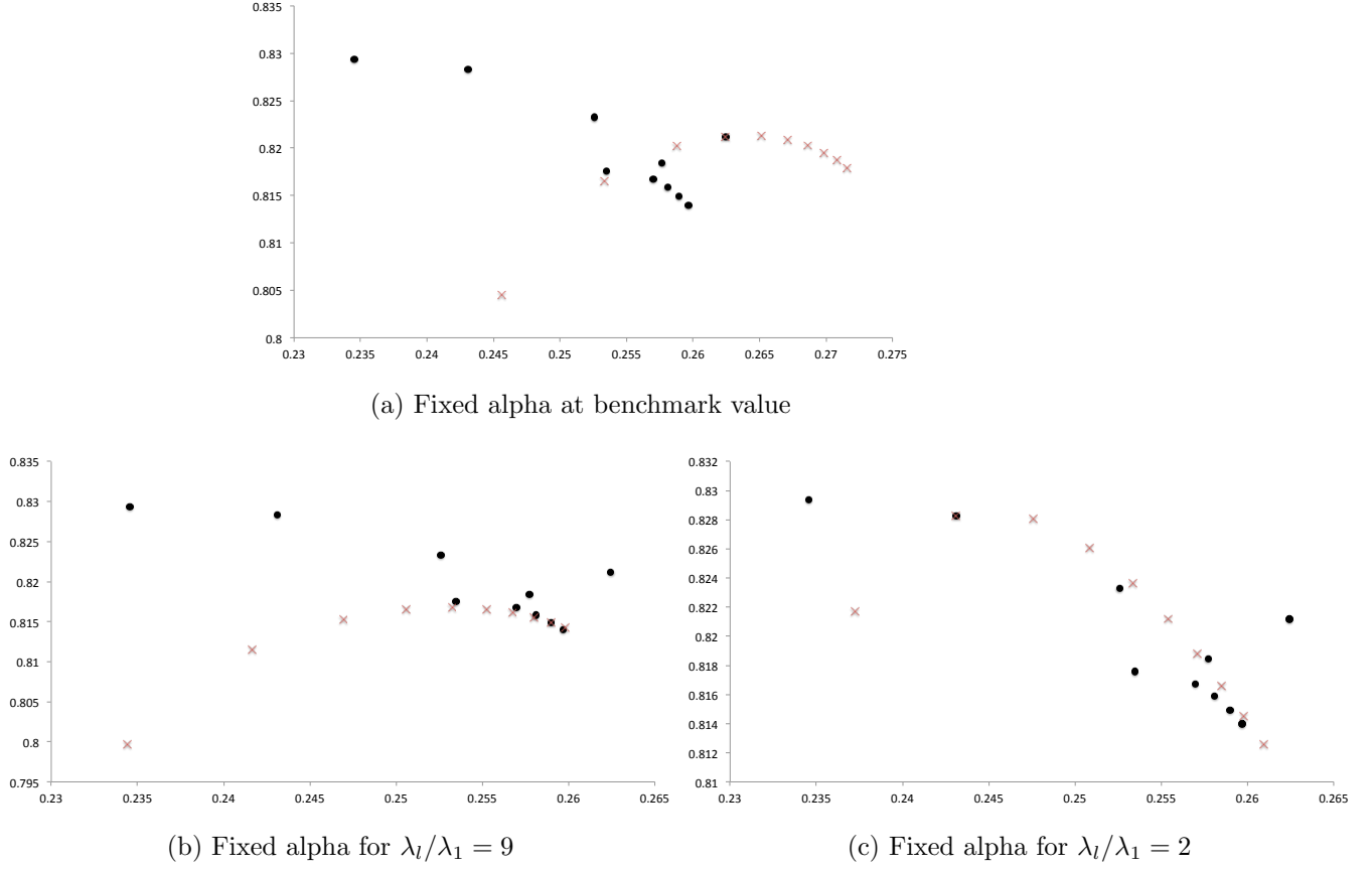
Figure 12: Aggregate price informativeness and concentration of institutional ownership with varying \lambda_l/\lambda_1
