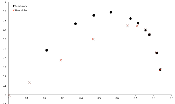
(c) Fixing information when \lambda_0 = 0.05
