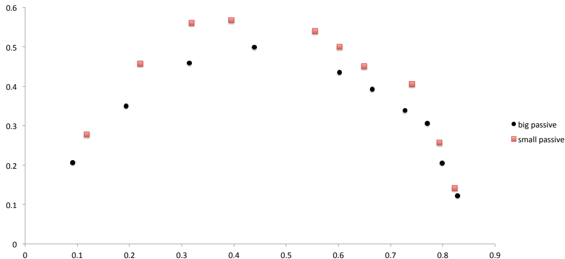
Figure 10: Aggregate price informativeness and institutional ownership: The case of big or small passive investors
