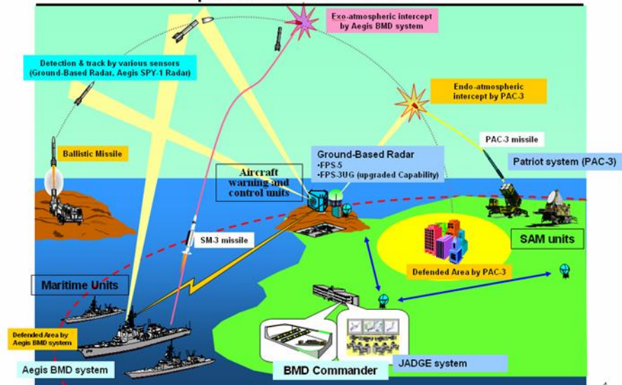
Japan's BMD Architecture
