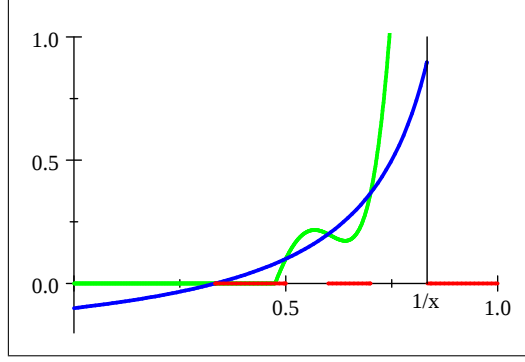
Figure 1. The figure illustrates the function v(\omega) (in light green) and the function D + \frac{N(\omega)}{1-\omega} (in blue). The bank's ideal investment rule is to invest when the state \omega is in the red intervals. This happens when either (i) \omega \geq \frac{1}{x} , so the project has positive NPV; or (ii) \omega < \frac{1}{x} , and the green line is below the blue line.
