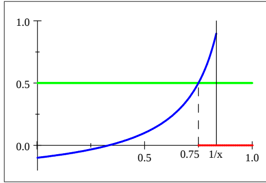
Figure 2. The figure illustrates the function v(\omega) (in light green) and the function D + \frac{N(\omega)}{1-\omega} (in blue) when D = 0.9 , x = 1.2 , and v(\omega) = 0.5 . The bank's ideal investment rule is to invest when \omega \geq 0.75 .
